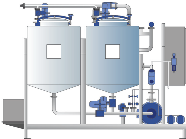
Typical single containment skid
